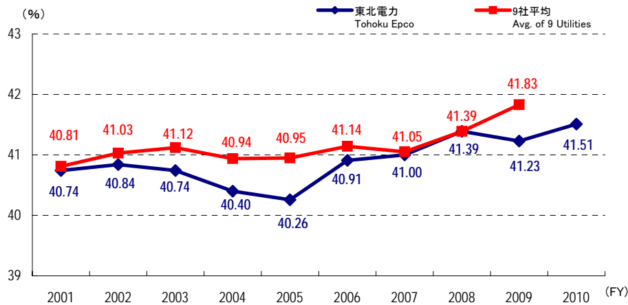
(5) 火力発電熱効率(発電端) Thermal Efficiency (at generation end)
