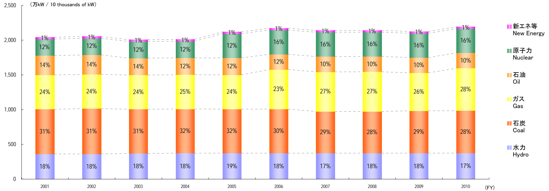
(1) 電源構成比の推移(含他社受電) Generating Capacity by Energy Source (including purchased power)
